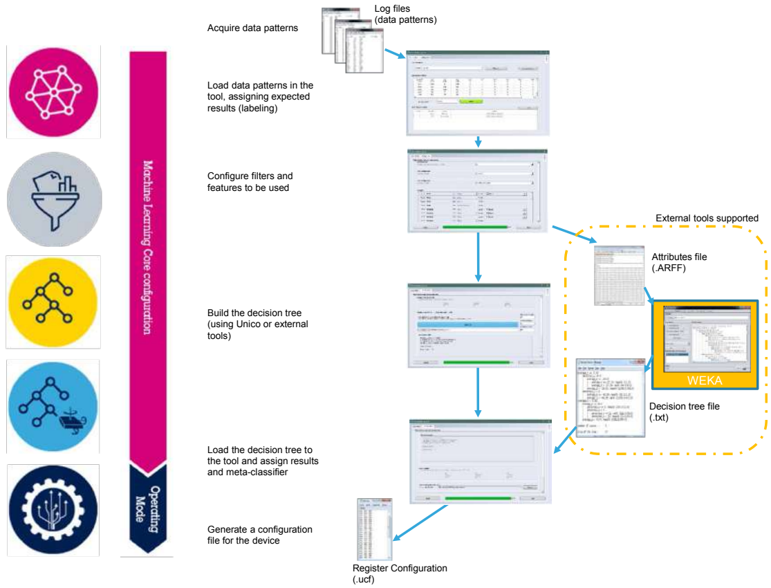
Figure 27. Configuration procedure
