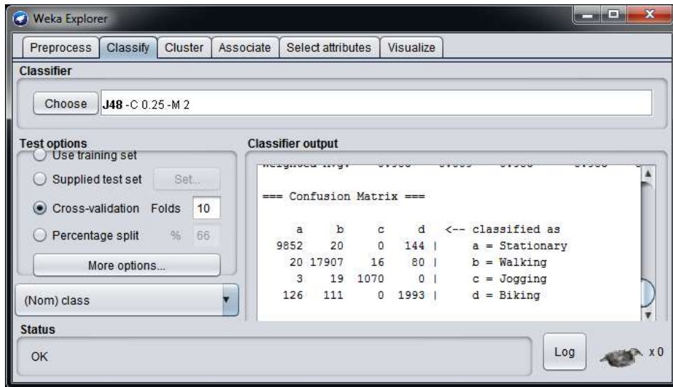
Figure 55. Confusion matrix
