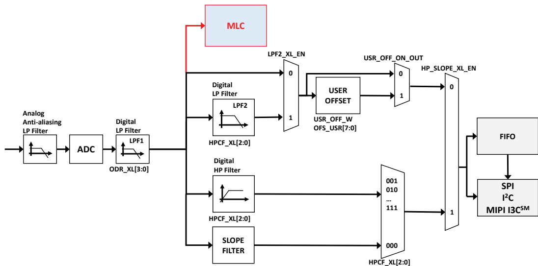
Figure 4. MLC inputs (accelerometer)
