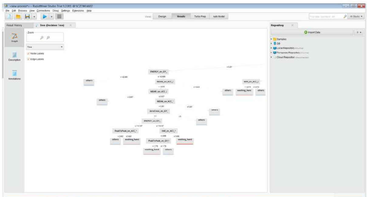
Figure 60. RapidMiner Studio - Decision Tree graph
