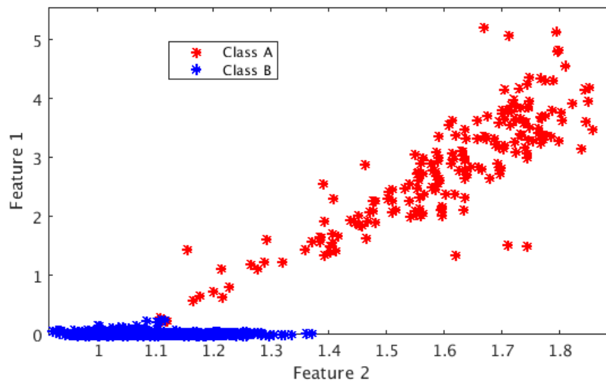
Figure 17. Visualization of two features and two classes
