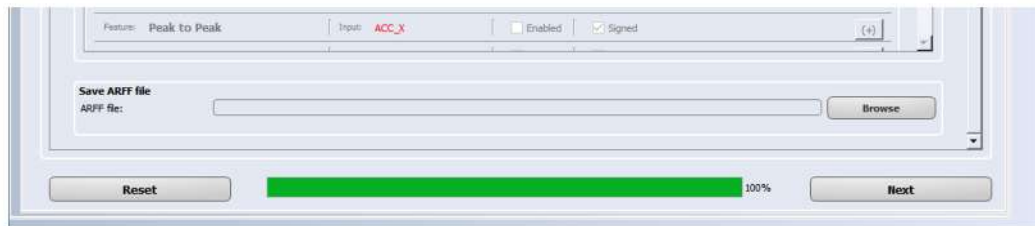
Figure 32. ARFF generation
