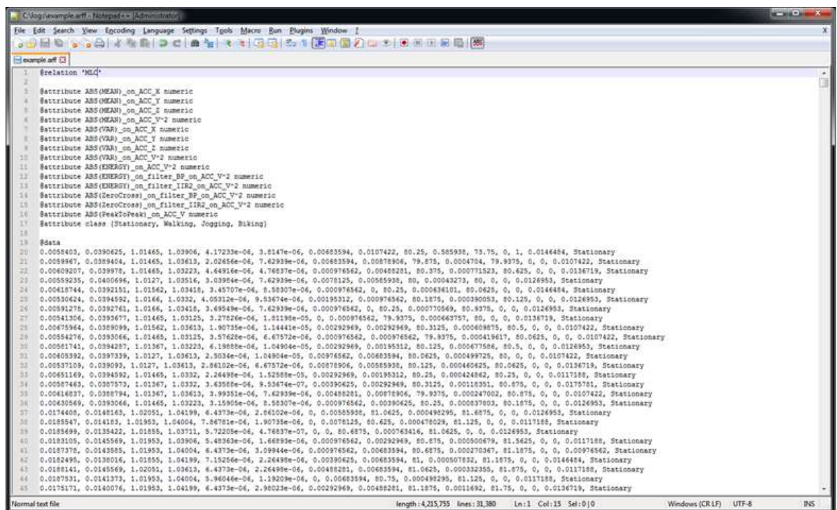
Figure 33. ARFF file
