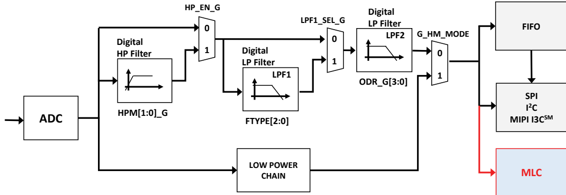
Figure 5. MLC inputs (gyroscope)
