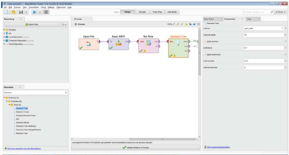
Figure 59. RapidMiner Studio - Decision Tree operator
